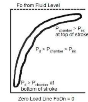
Figure 6 – Well dynamometer map with gas shutoff problem
