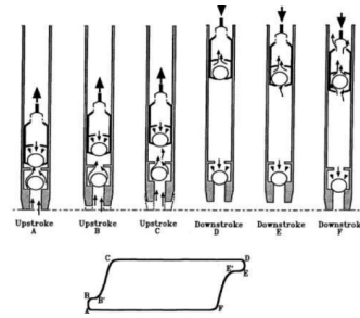
Figure 8 – Downhole dynamometer with a fault in the pipeline anchor
