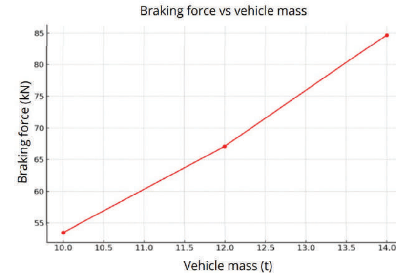
Figure 4 – Dependence of braking force on vehicle mass
