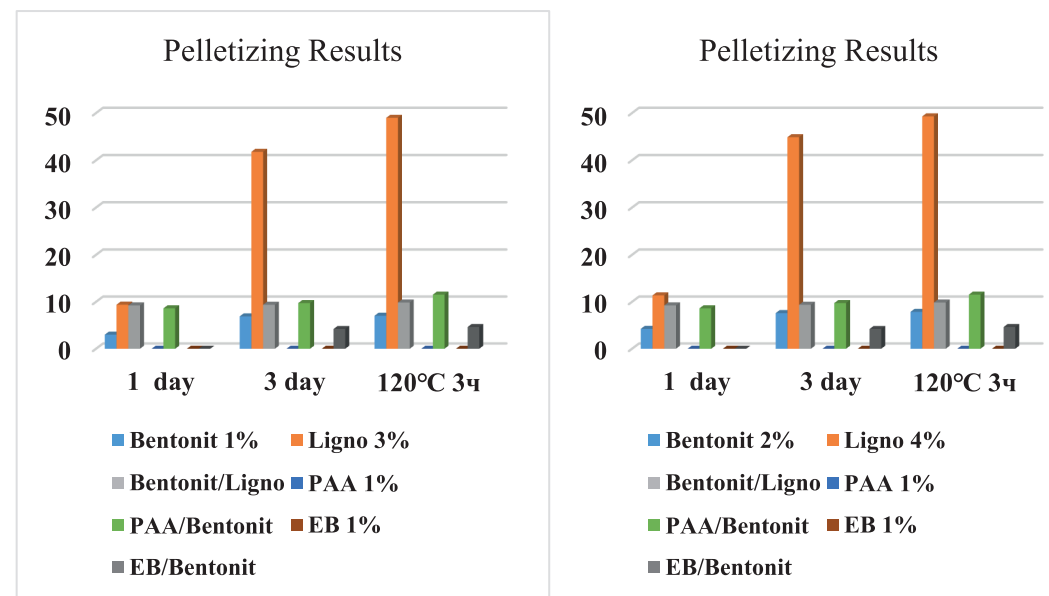
Figure 2 – Pelletizing Results for Materials № 1, № 2 and № 3
