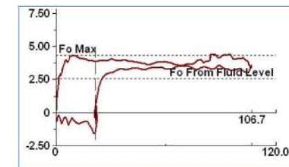
Figure 12 – Downhole dynamometer with clogged pump inlet
