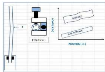
Figure 9 – Downhole dynamometer card with polished stem bend
