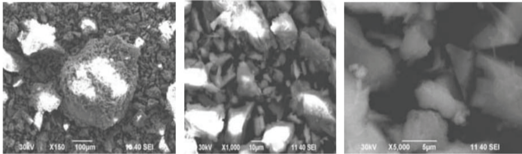
Figure 5 – Structure of Electric Arc Furnace Slag under a Scanning Electron Microscope
