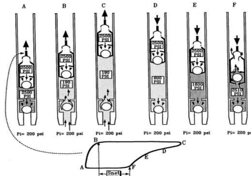
Figure 2 – Well dynamometer map with free gas influence problem
