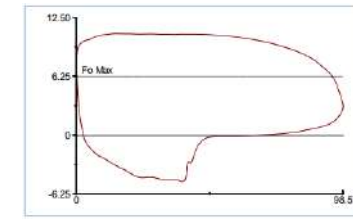
Figure 10 – Well dynamometer map with viscous oil
