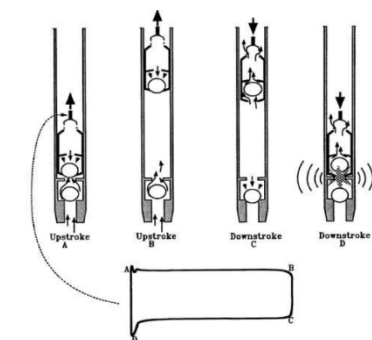
Figure 7 – Downhole dynamometer card with plunger kick problem
