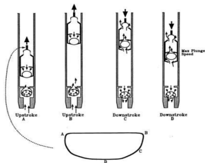
Figure 5 – Well dynamometer with a leakage problem of the receiver valve
