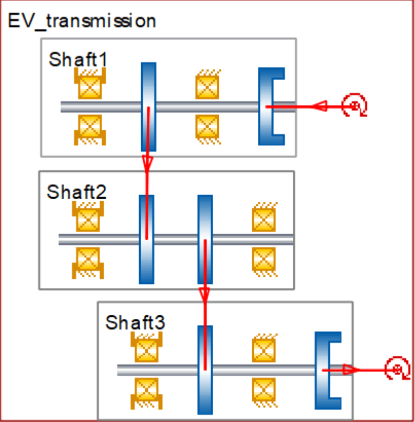
Figure 1 – Kinematic scheme of EV transmission
