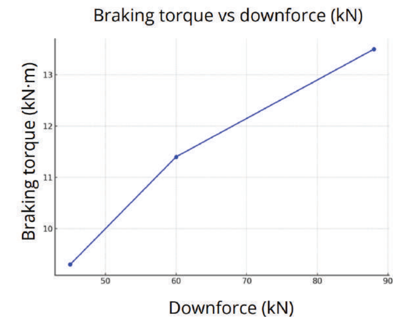
Figure 5 – Dependence of braking torque on pressing force
