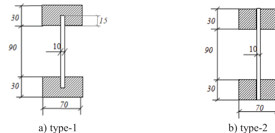
Figure 1 geometry of I-beams (all measurement in mm)
