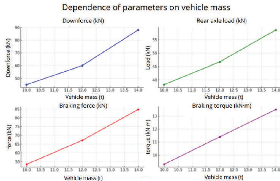
Figure 3 – Dependence of Downforce, Rear Axle Load, Braking Force, and Braking Torque on Vehicle Mass
