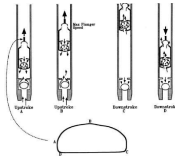
Figure 4 – Well dynamometer chart with track valve leakage problem
