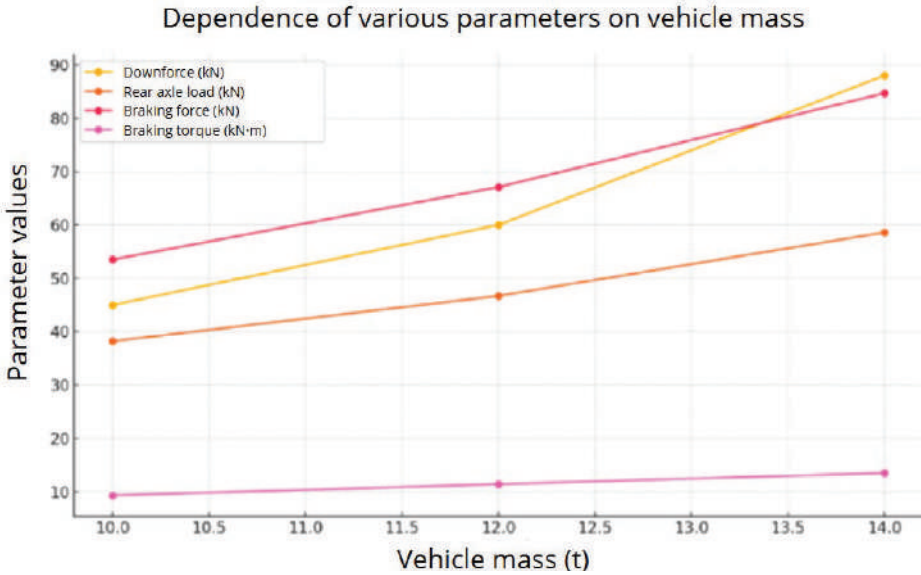
Figure 2 – Dependence of various parameters on vehicle mass
