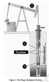
Figure 2 – Mechanical system of the pump
