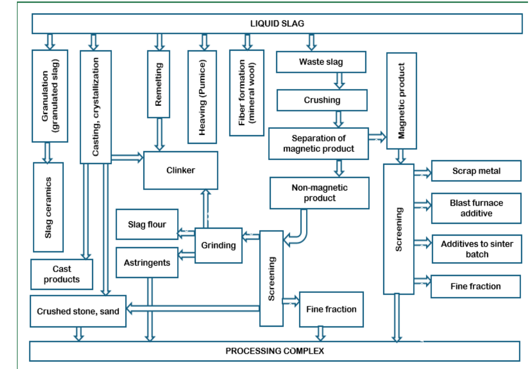
Figure 3 – Flowchart of Blast Furnace Slag Processing
