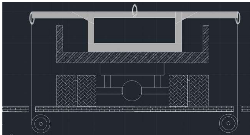
Figure 1 – Design proposed for loading brake tester rollers
