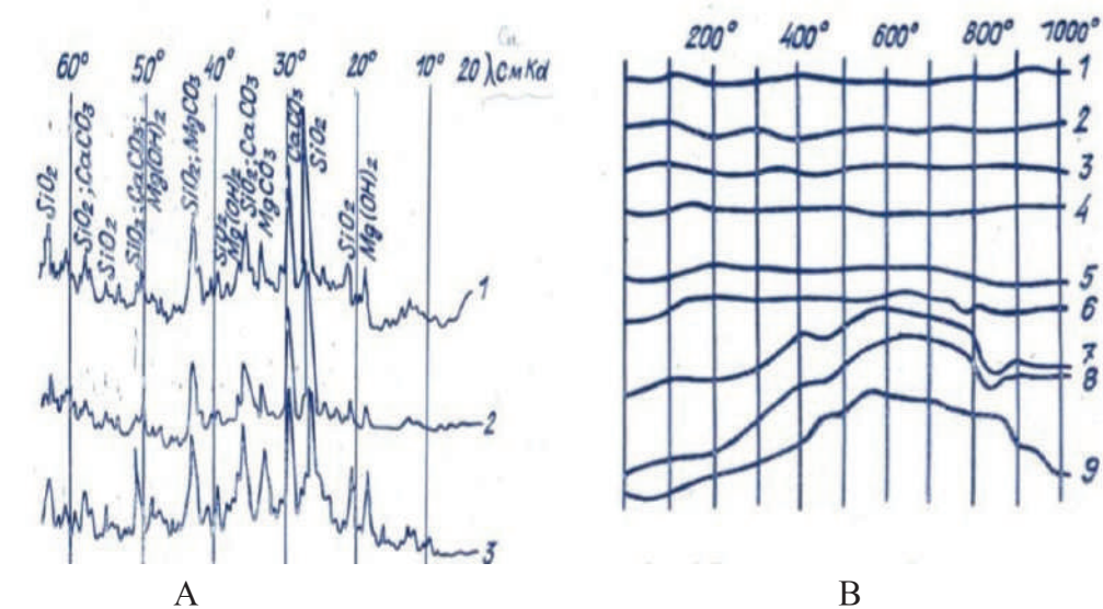
Figure 3 – A – X-ray Diffraction Patterns of Hydrated Fines from Crushed Stockpiled Open-Hearth Slag at the Ages of: 1 – 1 day; 2 – 1 year; 3 – 2 years [14].
