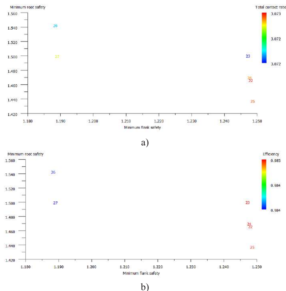
Figure 4 – Graphs of the dependence of minimum root safety on minimum flank safety for the general contact ratio (a) and for the efficiency (b) of the second speed gear pair
