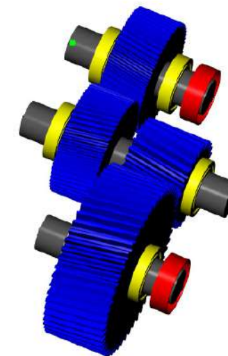
Figure 6 – 3D model of the electric vehicle gearbox
