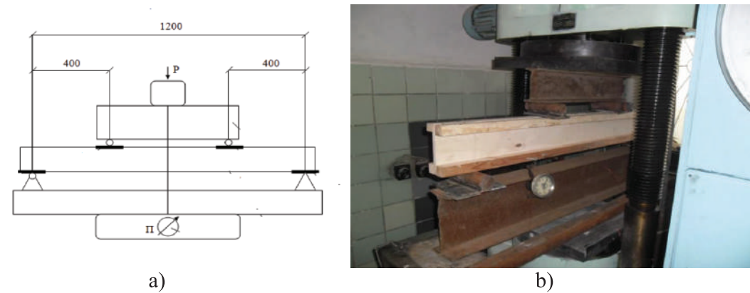
Figure 2 – Test setup a) test setup (all measurement in mm); b) actual test setup
