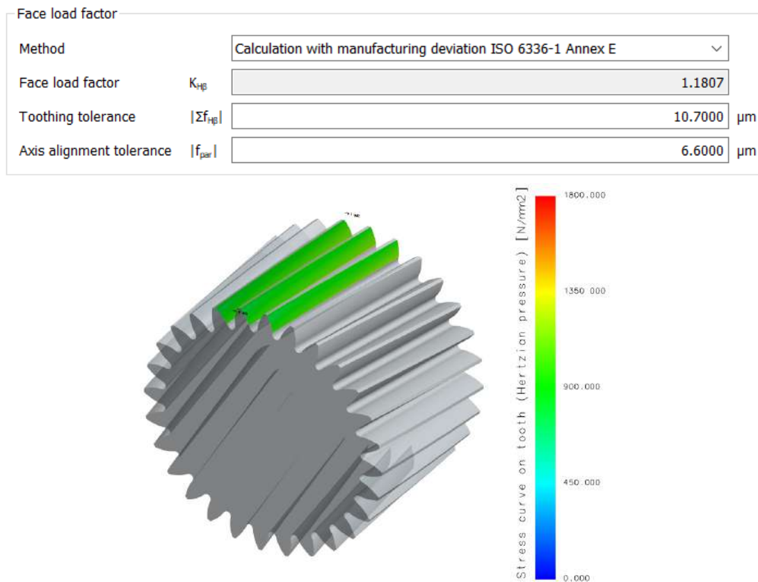
Figure 10 – (a) Load distribution factor along the tooth length K_{H\beta} calculated considering manufacturing deviations according to ISO 6336-1 Annex E.(b) Contact stress distribution
