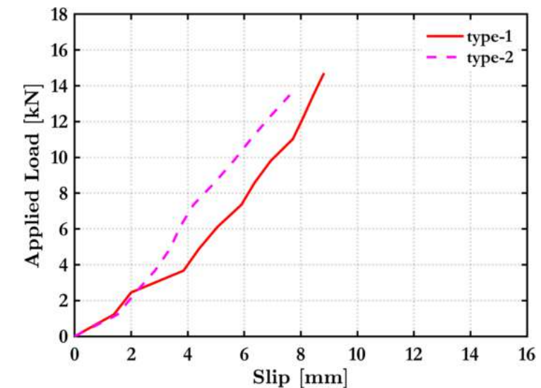
Figure 3 – Load displacement plot
