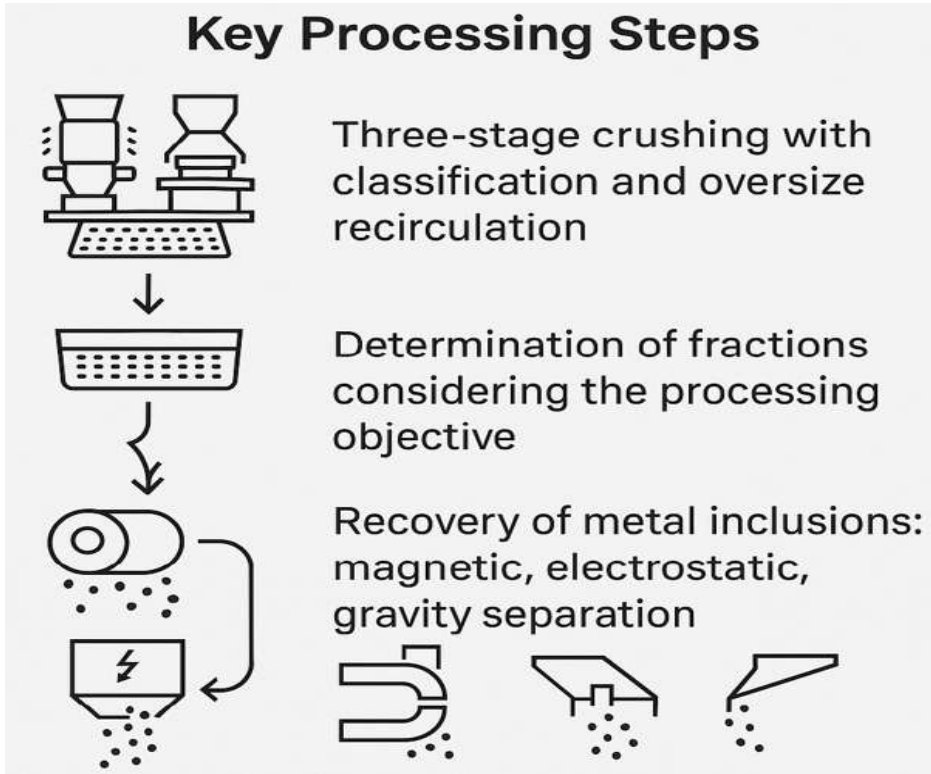
Figure 2 – Flowchart of Mechanical Processing of Metallurgical Slags Highlighting Key Stages and Equipment
