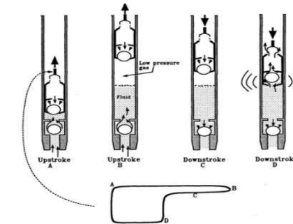
Figure 3 – Downhole Dynamometer card with liquid impact problem
