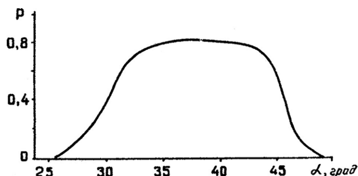
Figure 1 – Probability P of avalanche formation on various slope steepness \alpha with the snow height of 100 cm
