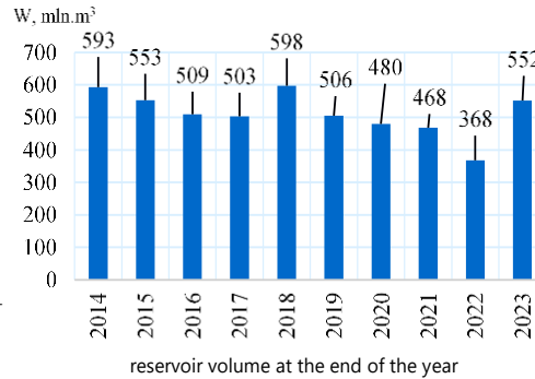
Fig. 2: Dynamics of changes in the components of the water balance of the Verkhnetobolskoye reservoir
