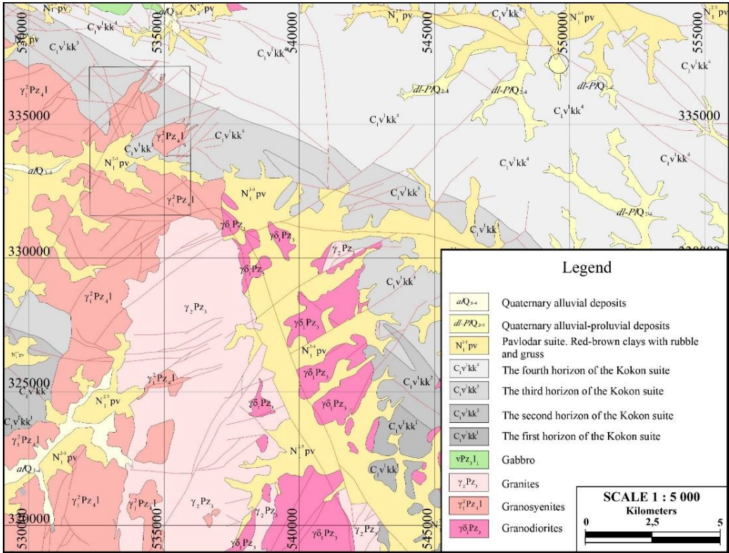
Fig. 3: Geological map of the Verkhnee Espe deposit, scale 1:5000.
