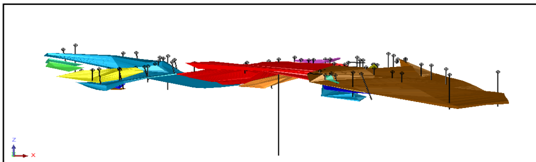
Fig. 5: Framework model of the ore bodies of the Verkhnee Espe deposit in Surpac software, clearly showing the distribution of ores in 3D space.
