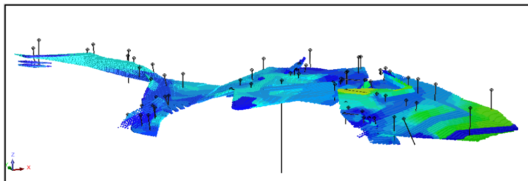
Fig. 6: Block model of the ore bodies of the Verkhnee Espe deposit in Surpac software, showing the distribution of rare earth element content in the ore bodies, ranging from blue to yellow.
