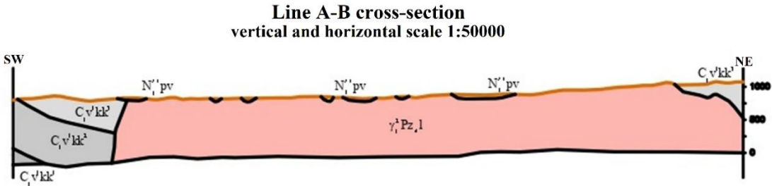
Fig. 4: Geological section of the Verkhnee Espe deposit along the A-B line, scale 1:50,000.
