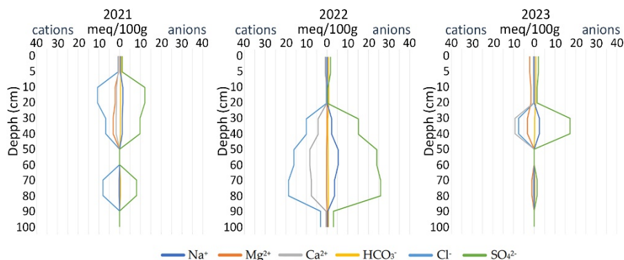
Figure 6. Salt profile presenting variability of the anionic and cationic compositions in the total amount of salt (P-27).
