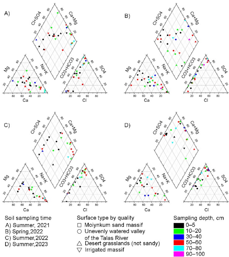
Figure 5. Piper diagram presenting the distribution of anionic and cationic compositions of the soils.
