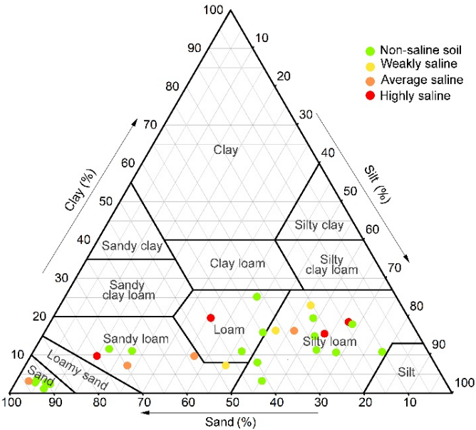
Figure 2. Soil texture triangle showing classified samples (salinity levels) from Talas district ecosystems.
