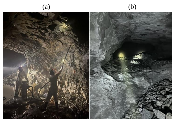
Figure 9. Experimental-industrial tests of breaking thin slope ore bodies in the Akbakai mine using charges with controllable blast characteristics
