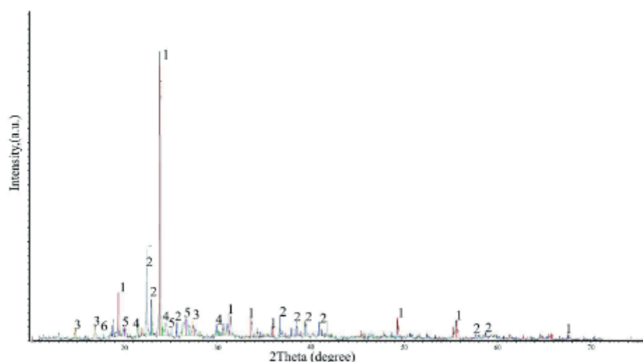
Figure 3 – Diffractogram of the Sample from One of the Deposits in Kazakhstan
