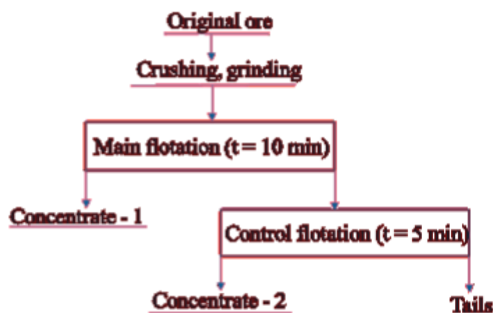
Figure 5 - Flotation scheme
