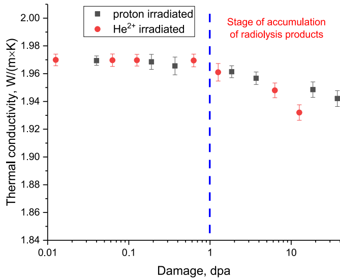
Fig. 6. Results of comparative analysis of alterations in the thermal conductivity coefficient of the studied ceramics when irradiated with protons and He 2+ ions.
