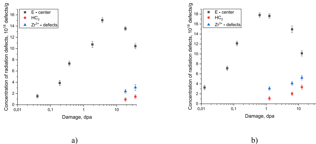
Fig. 3. Assessment results of the concentration of various defects in the damaged layer depending on the irradiation type: a) proton irradiation; b) \text{He}^{2+} ion irradiation.
