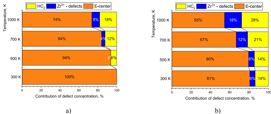
Fig. 8. Assessment results of the weight contributions of different types of defects in the damaged layer depending on the irradiation temperature, characterizing the change in the degradation kinetics due to thermally stimulated diffusion of radiation defects: a) proton irradiation; b) \text{He}^{2+} ion irradiation.
