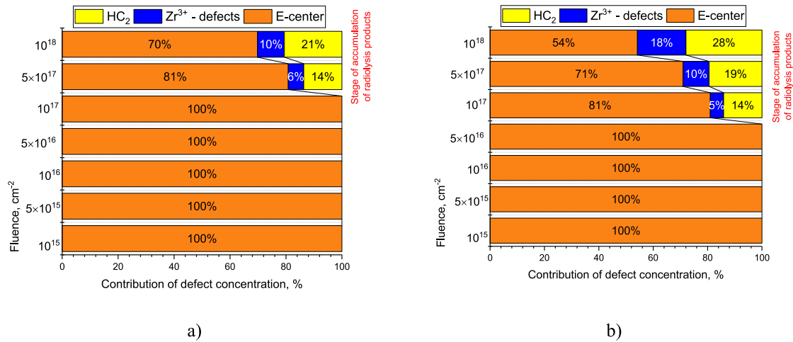
Fig. 5. Assessment results of the weight contributions of various defects in the damaged layer depending on the irradiation fluence in the case of irradiation of ceramics with different radiation types: a) proton irradiation; b) He 2+ ion irradiation.
