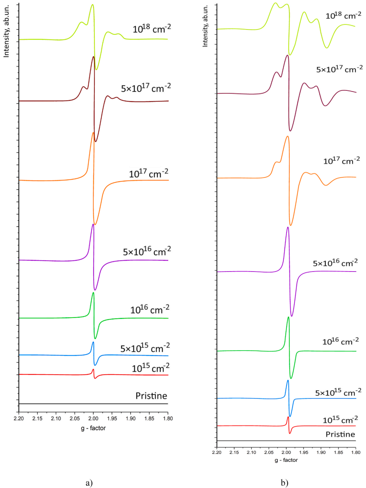
Fig. 1. EPR spectra of ceramics depending on the irradiation fluence: a) proton irradiation; b) \text{He}^{2+} ion irradiation.
