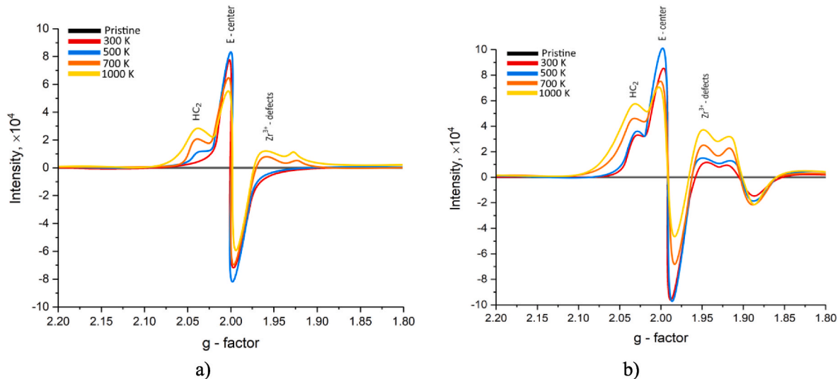
Fig. 7. Results of EPR spectroscopy of the studied ceramic samples exposed to irradiation at a fluence of 10^{17} \text{ cm}^{-2} with a change in irradiation temperature: a) proton irradiation; b) \text{He}^{2+} ion irradiation.
