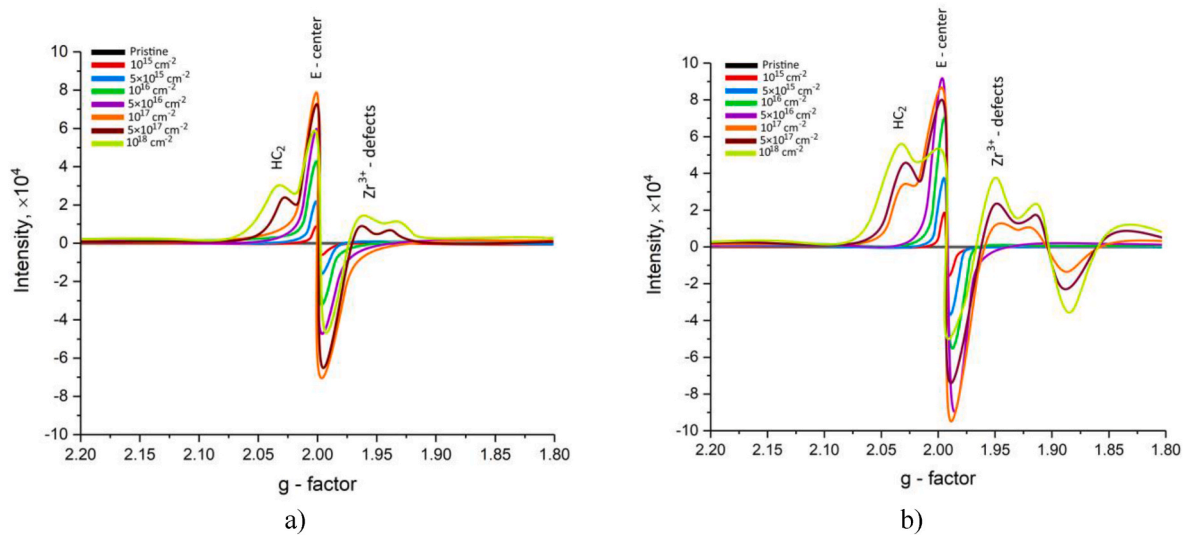
Fig. 2. Comparative analysis results of alterations in the intensities of the EPR spectra of the studied ceramics depending on the type of irradiation, reflecting the damaged layer degradation kinetics: a) proton irradiation; b) \text{He}^{2+} ion irradiation.
